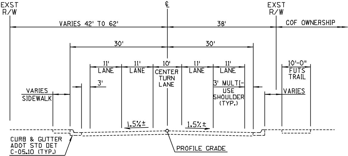
TYPICAL SECTION ROUTE 66 EXISTING ROADWAY
