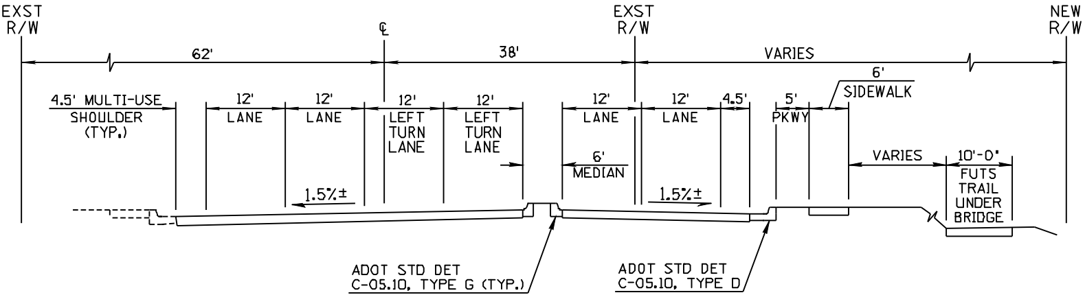
TYPICAL SECTION ROUTE 66 EAST OF LONE TREE ROAD
