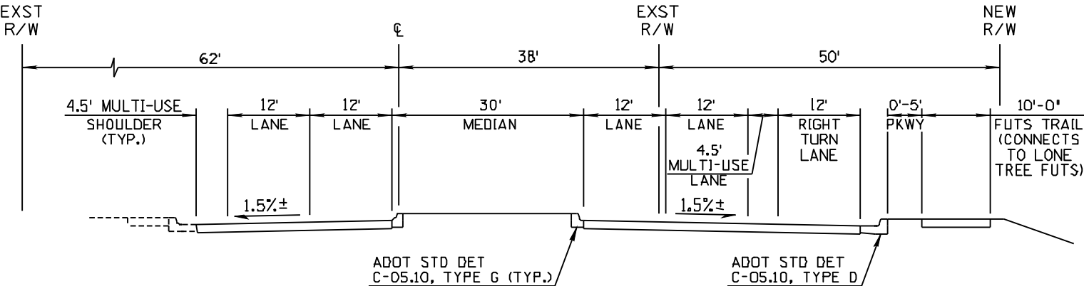
TYPICAL SECTION ROUTE 66 WEST OF LONE TREE ROAD
